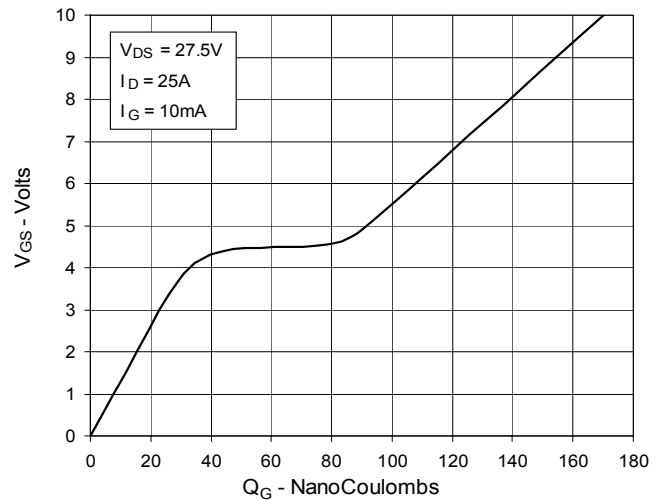
Fig. 10. Gate Charge
